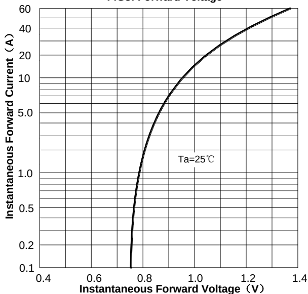
FIG3: Forward Voltage
